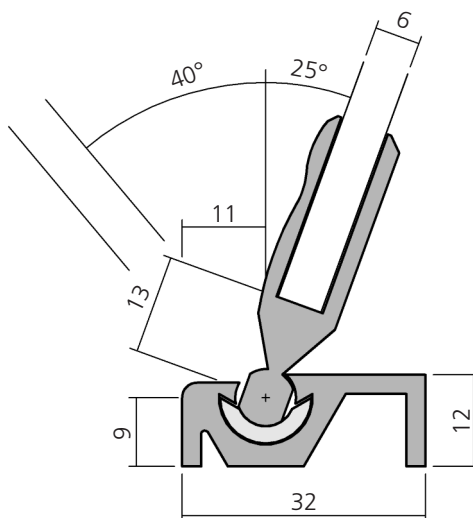
Anschlagprofil, Aluminium Stop profile
